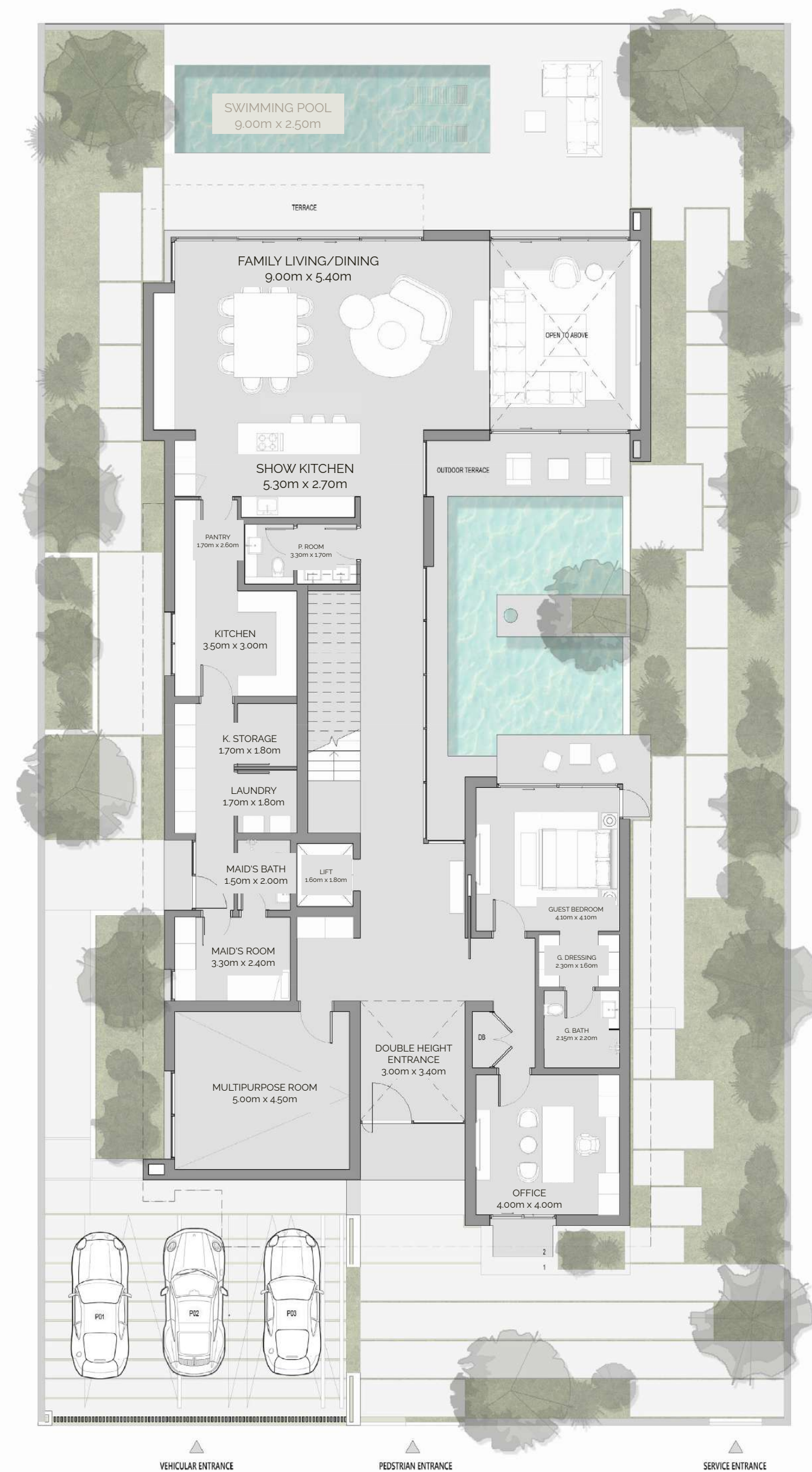
GROUND FLOOR
